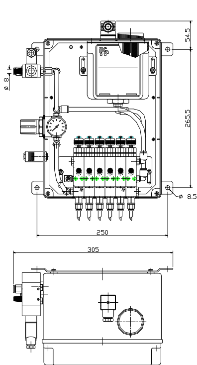
DIMENSIONS UCSG-SE
